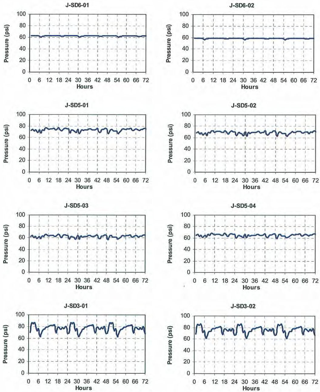
Figure F-2. Suncreek Nodes Pressure Curves - Max Day, Water Supply Scenario 6
